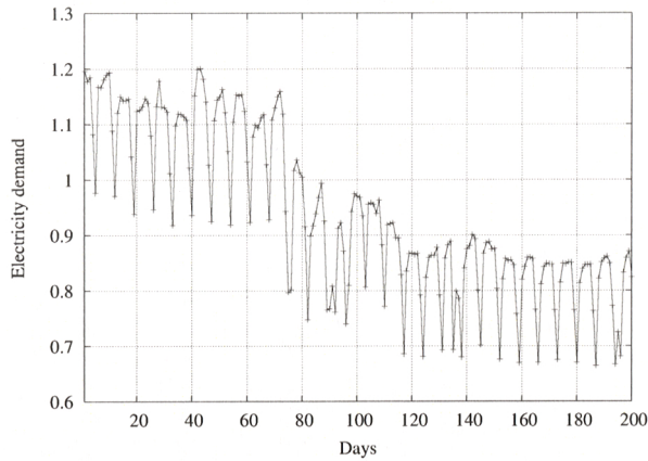
Fig. 6. PolElec: test series (201 samples).
