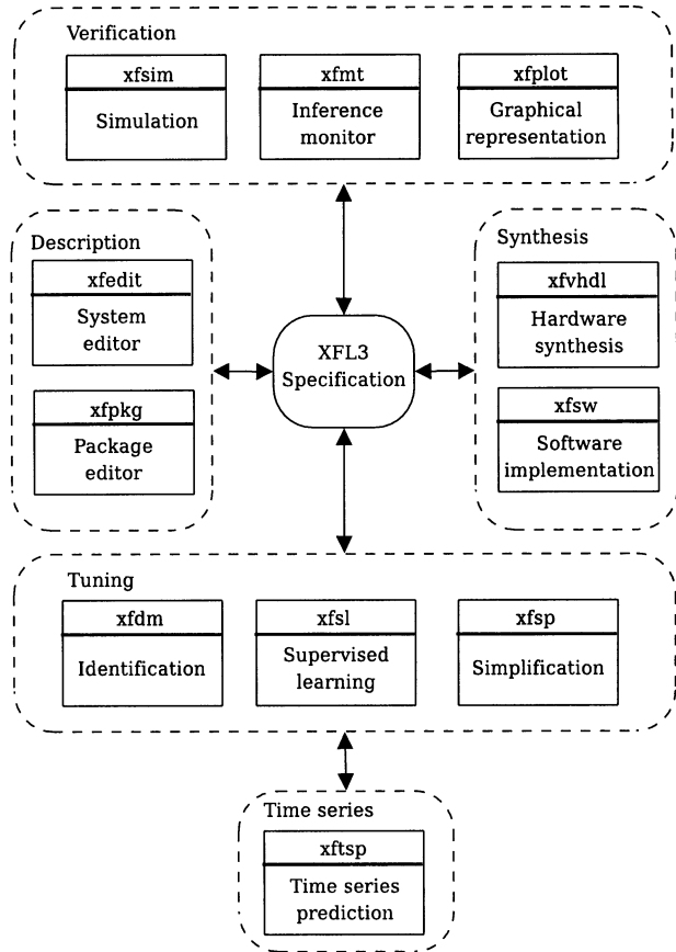
Fig. 2. Overall component architecture of Xfuzzy.
