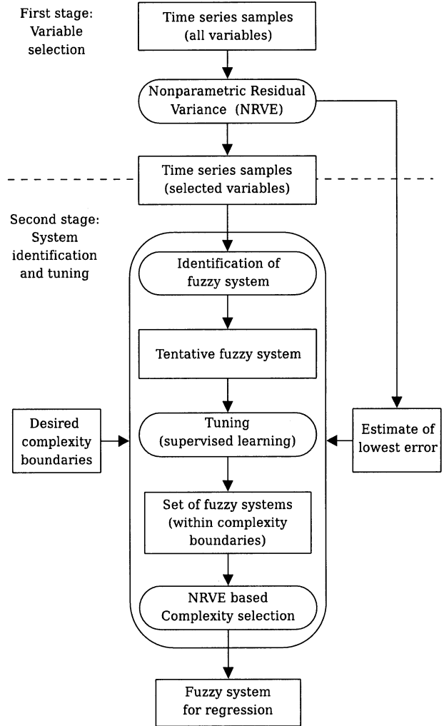
Fig. 1. Methodology Framework of xftsp .
