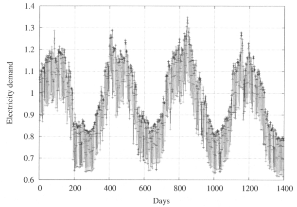
Fig. 5. PolElec: training series (1400 samples).
