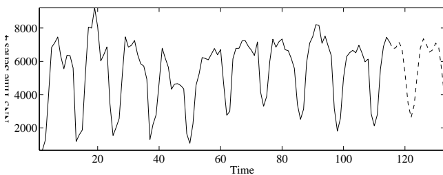
Fig. 14. Prediction of the 4 th time series. Solid line represents the known time series and the dashed one the prediction.
