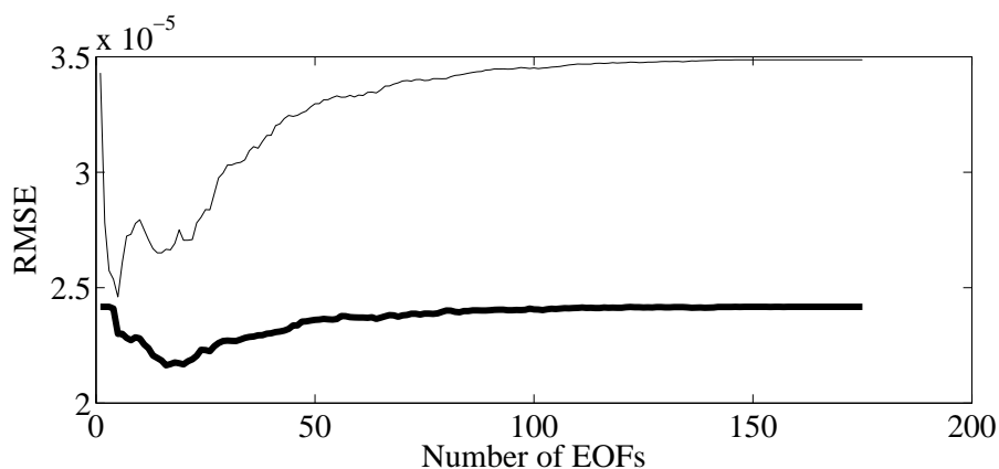
Figure 11. Validation Errors with Respect to Number of EOFs with the Plain Column Mean Initialization. The fine grey line and the bold black line represent the error of the EOF and the SOM+EOF, respectively. Source : SnP ; European Fund Weekly Return (07/11/2003 to 27/10/2006). Computation from the Authors.
