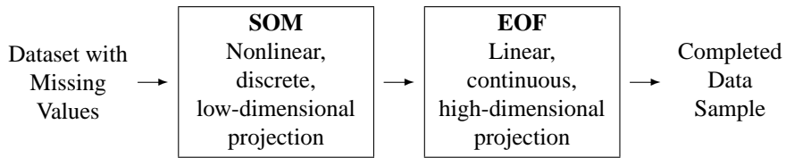
Figure 1. Global methodology, the SOM+EOF, summarized.
